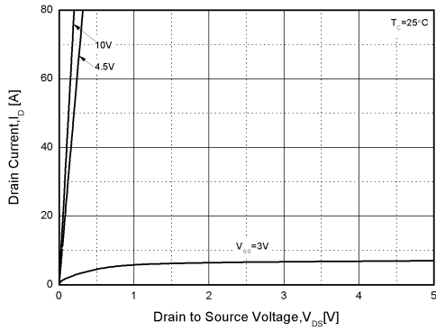
Figure1. Output Characteristics
