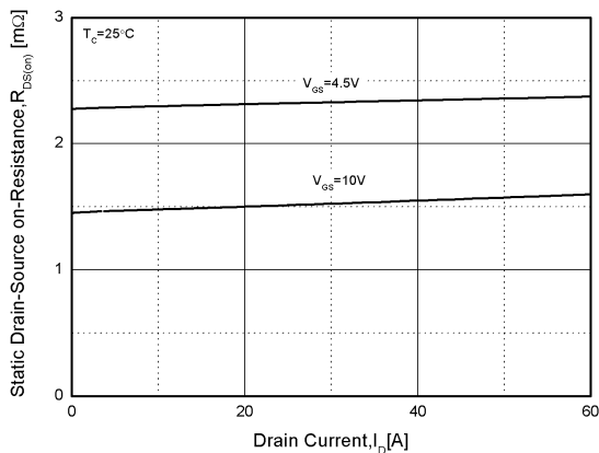
Figure3. Rdson-Drain Current
