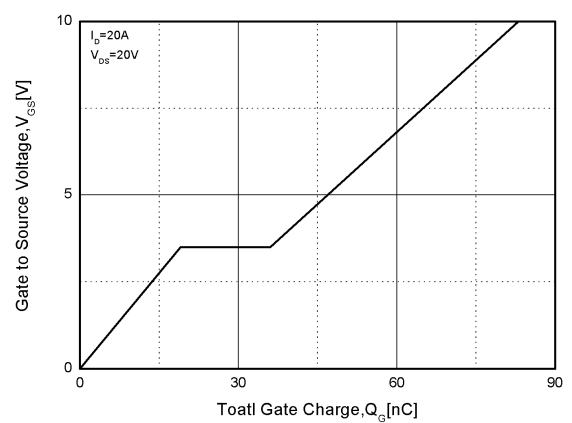
Figure6. Gate Charge
